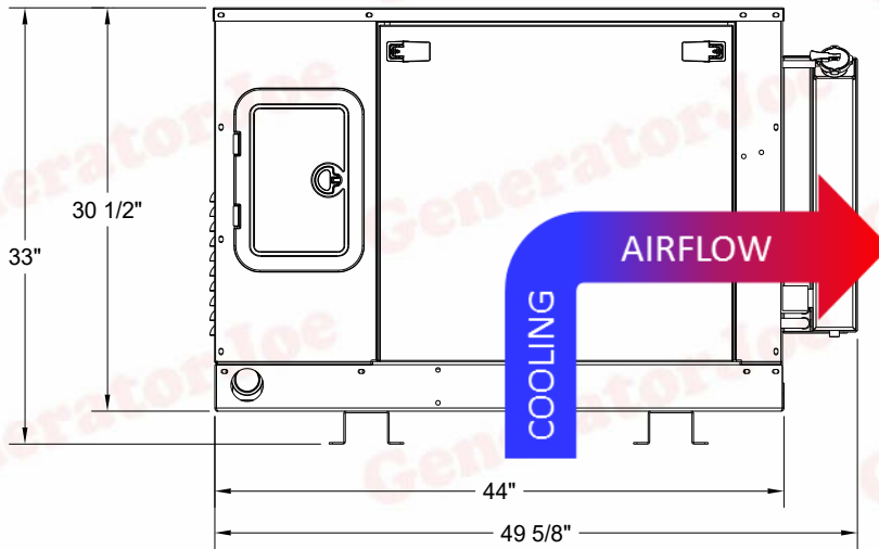
Air Flow
